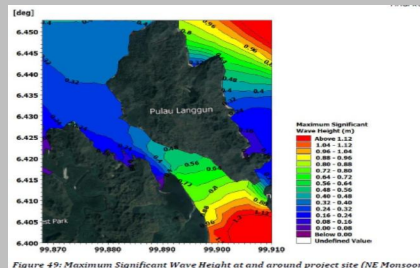
Figure 49: Maximum Significant Wave Height at and around project site (NE Monsoon)
