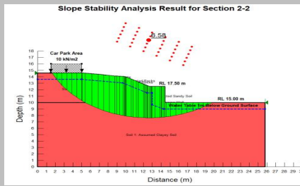
Slope Repair Design at IPD Lahad Datu, Sabah
