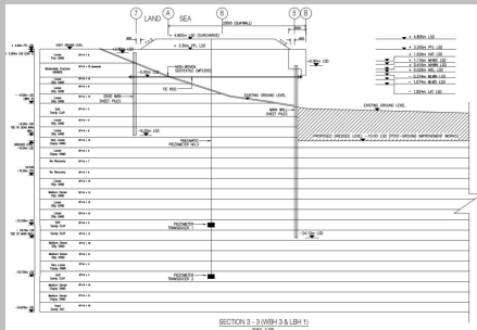
Geotechnical Stability Check, Lumut Naval Base Jetty Extension, Perak
