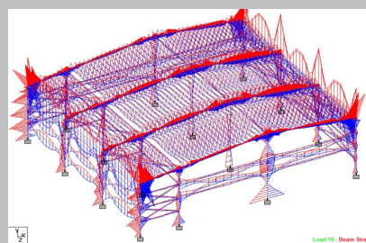
Steel Portal Frame Building, Alor Setar Kedah
