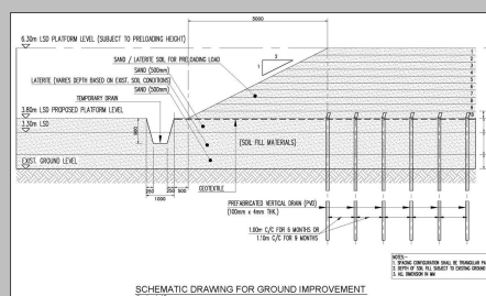
Ground Improvement Works, RKAT, Pulau Indah, Klang
