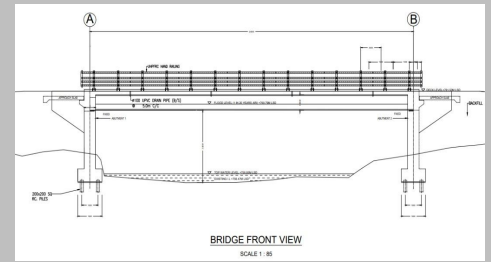
Melout Bridge, Tambunan, Sabah
