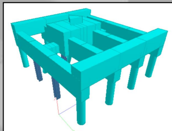
Bollard Capacity Assessment, Labuan
